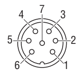
Solder side 7P Male socket to 7" Display
